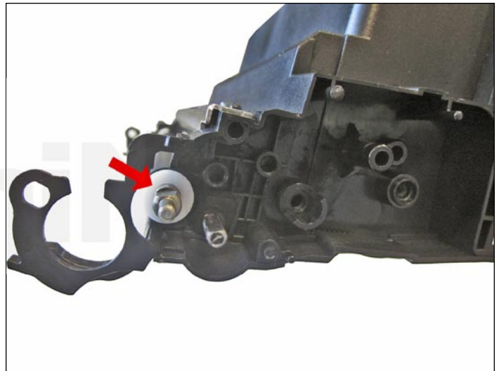
29. Replace the bushings on both side of the developer roller.
