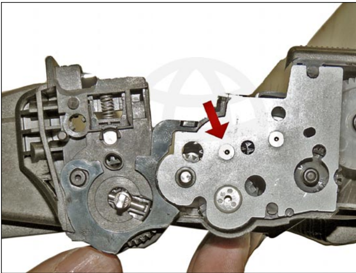
31. Install the gear axle plate.
