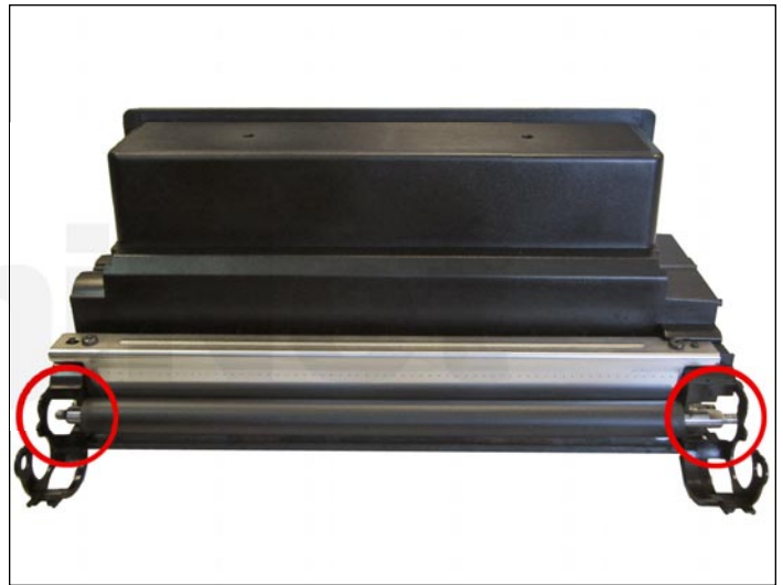
27. Clean the developer roller with a dedicated developer roller cleaner, and replace into the hopper. Place the long shaft side to the gear side of the cartridge. It should snap in place if installed correctly.
