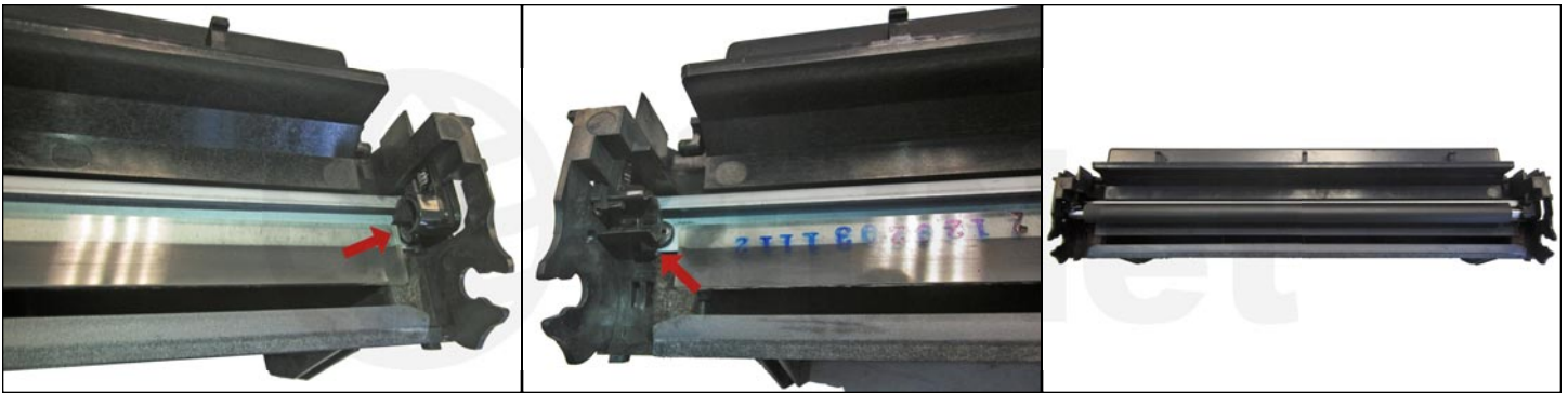
15. Install the PCR holders.
