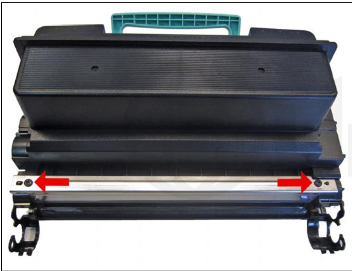
26. Install the doctor blade and two screws.
