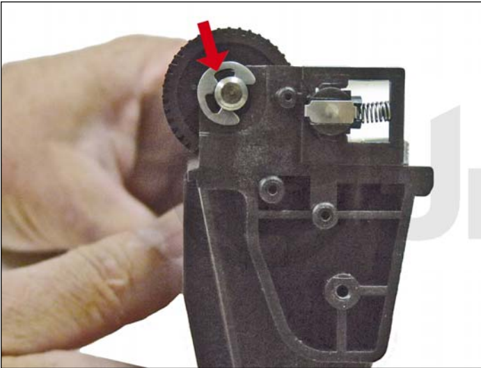
22. On the waste hopper, remove the E-ring from the drum axle.
