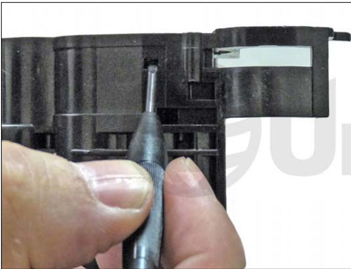
12. On the fill plug side, press in on the plastic tab and remove the spring/plastic bushing assembly.
