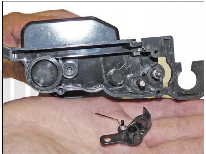
12. On the fill plug side, press in on the plastic tab and remove the spring/plastic bushing assembly.
