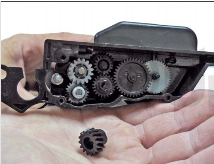
11. Remove the developer roller drive gear, and place a strip of tape across the remaining gears.
