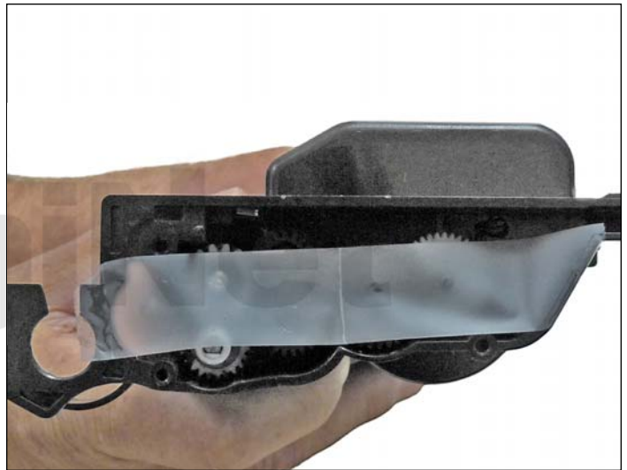
11. Remove the developer roller drive gear, and place a strip of tape across the remaining gears.
